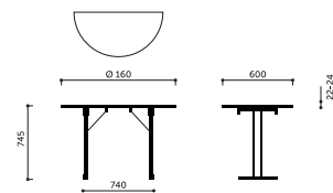
Standard Folding Table 4681-45
